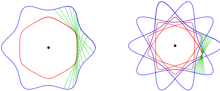
FIGURE 2. Self-Bäcklund curves (blue), with winding numbers 1 (left) and 3 (right). A line segment (green) moves with its end points sliding along the curve, forming a constant area triangle with the origin, while the midpoint of the line segment traces a curve (red), always tangent to the line segment at its midpoint. The two curves depicted here are members of an infinite family of self-Bäcklund curves described explicitly in Section 4 in terms of the Weierstrass \wp -function. For more images and animations, see [12].
